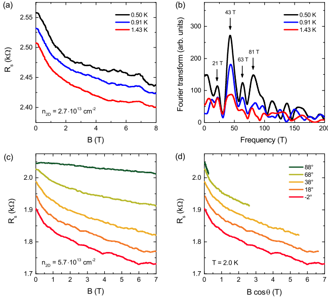
FIG. 4. (a) Sheet resistance R_s as a function of the magnetic field B applied in the out-of-plane direction for different values of T in a gated (111) diamond surface. Curves at T = 0.91 \text{ K} and T = 1.43 \text{ K} are shifted for clarity. (b) Fourier spectra of the B^{-1} -dependence of the oscillations shown in (a). Frequencies at 21 T, 43 T, 63 T and 81 T are highlighted by arrows. (c) R_s vs. B for another gated (111) diamond surface, for different angles \theta between B and the surface ( \theta = 0^\circ indicates that B is perpendicular to the surface). Curves at \theta = 18^\circ , \theta = 38^\circ , \theta = 68^\circ and \theta = 88^\circ are shifted for clarity. (d) Same data of (c) plotted vs. B \cos \theta , highlighting that the magnetotransport features depend only on the out-of-plane component of B . All data are adapted from Ref.46.
