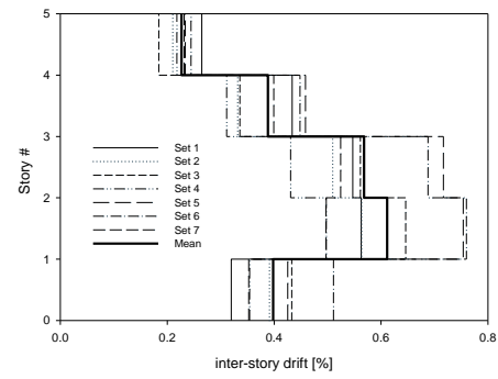
Figure 6. Inter-story drift of the seven groups of selected records compared with the mean values.
