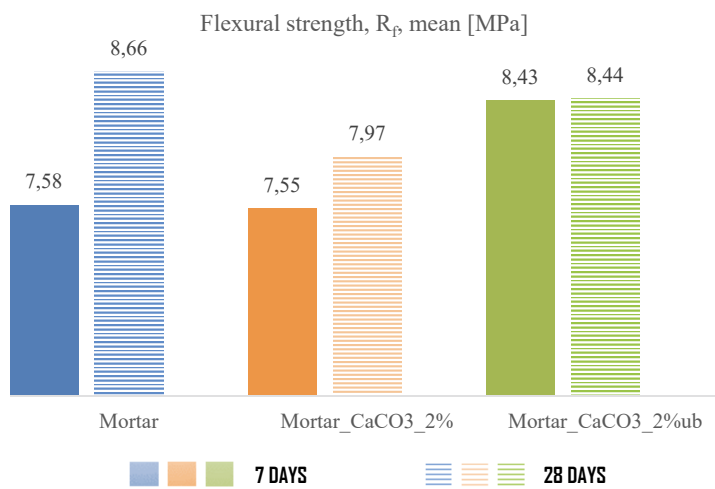
Figure 7: Flexural strength (mean value) after 7-28 days curing.
