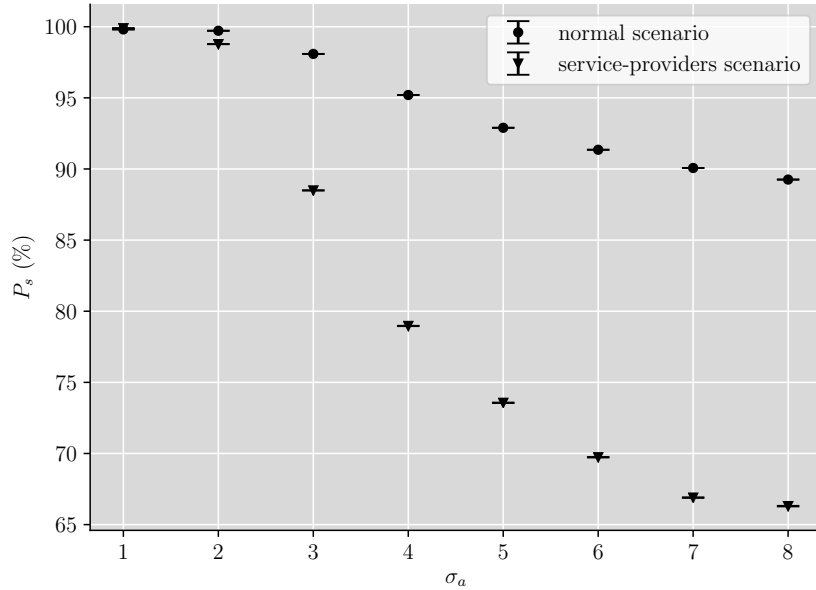
Figure 6.10: Payment success probability in the service-providers scenario in the LN mainnet.
