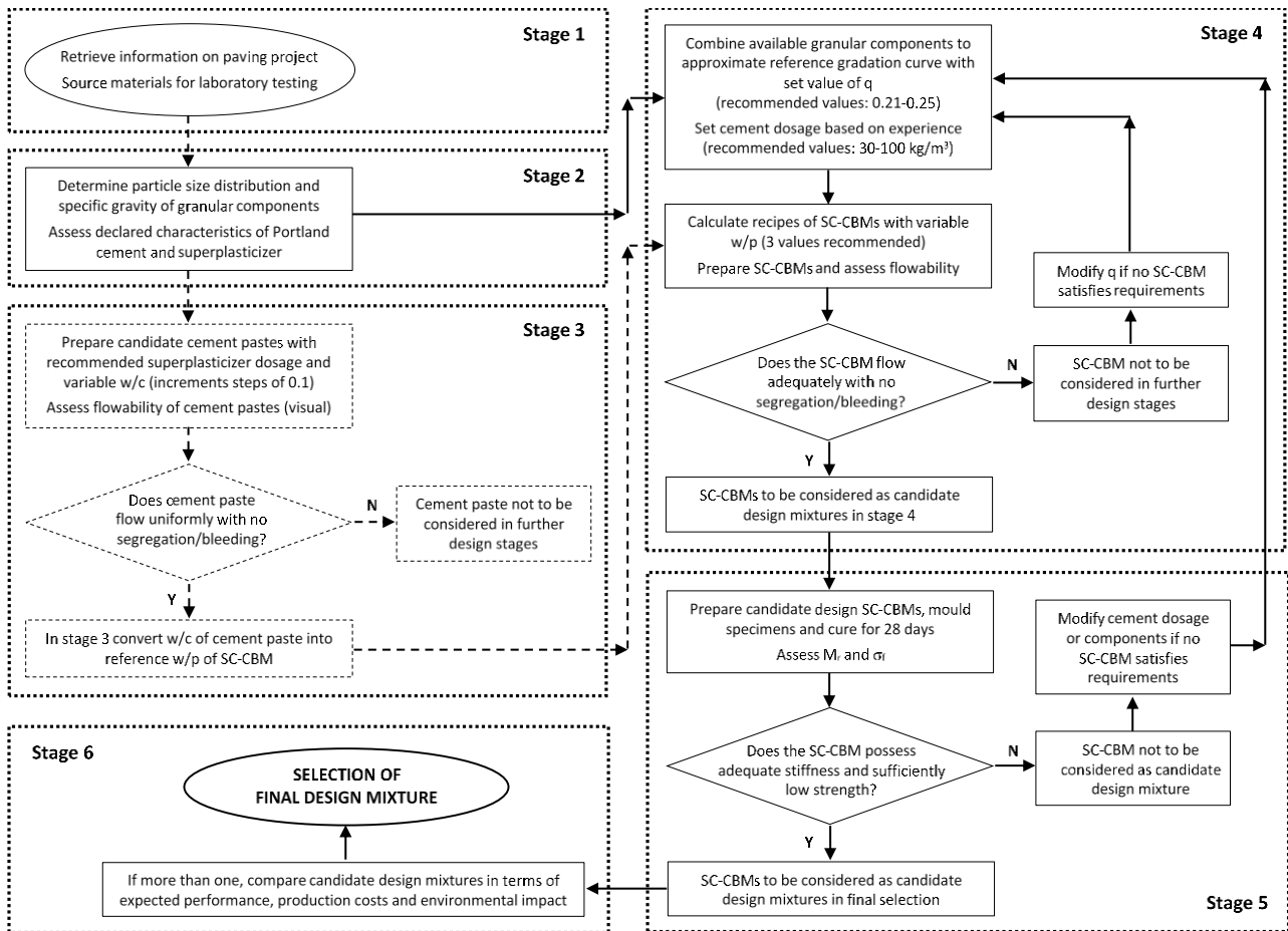
Fig. 7. Flow chart of the proposed mix design procedure
