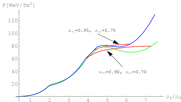
Figure 3: The same of Fig. 2 with the Gibbs construction (red lines) in region of the unstable EOSs.
