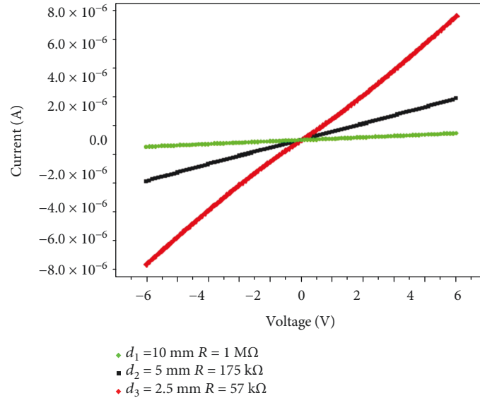
FIGURE 2: I-V characterizations performed on PEO/PEDOT:PSS nanofibers, obtained by providing three different distances between metallic strips: d_1 = 10 mm, d_2 = 5 mm, and d_3 = 2.5 mm.
