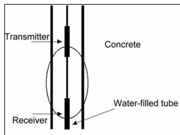
Figure. 3 – Zoom on the instruments disposition during acquisition.
