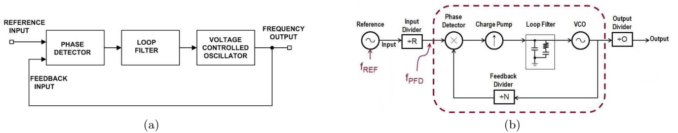
Fig. 3. Illustration to Subsection 2.2.3: the “minimal” PLL vs. a more general synchronization circuit
