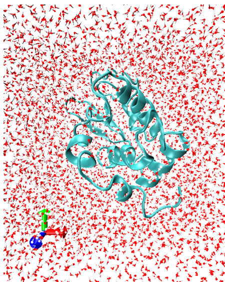
Fig. 9 Snapshot of the Lysozyme protein (PDB ID: 1AKI) solvated in water. The image has been created using the VMD software [26]. For the sake of clarity, water molecules at z > z_{max}/2 ( z_{max} = 7 nm) have been hidden in the current visualization. Color code: cyan, protein; red, oxygen atoms; white, hydrogen atoms.
