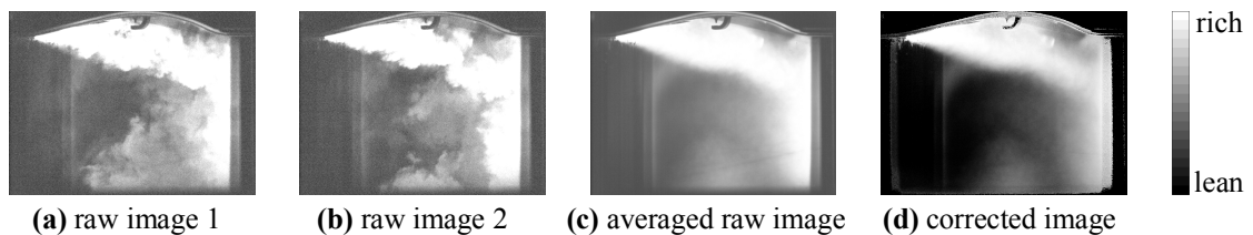
Figure 4.4 PLIF image processing procedure (intake on the lefthand side)
