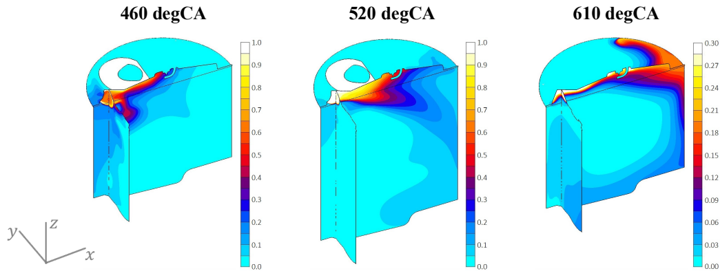
Figure 4.16 Numerical fuel mass fraction contours: 1500 rpm full-load, EOI = 600 degCA
