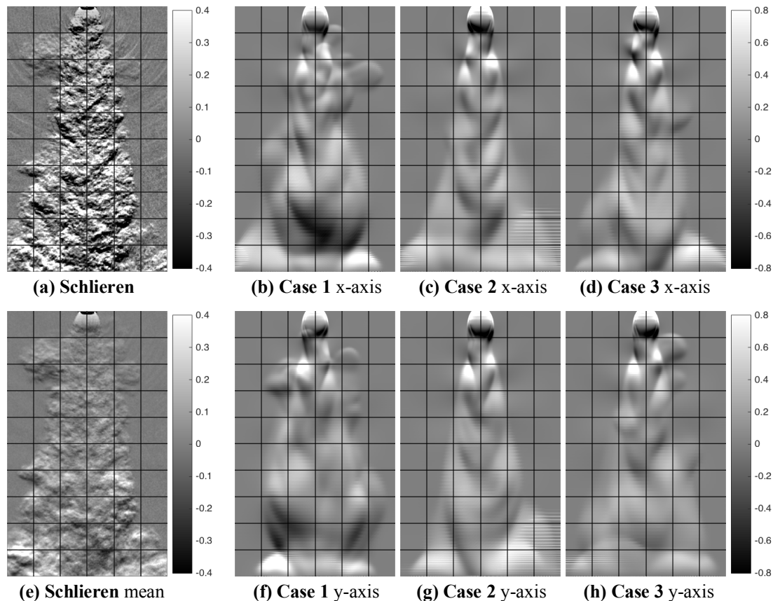
Figure 3.12 Comparison between the schlieren contrast and numerical result at 1800 \mu s
