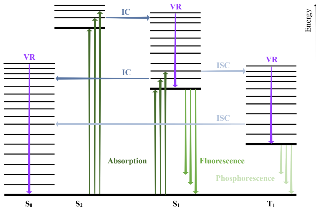
Figure 4.2 Jabłoński diagram of the LIF photophysical processes of excitation and relaxation of organic molecules in the ground state and three excited electronic states IC – internal conversion, ISC – intersystem crossing, VR – vibrational relaxation
