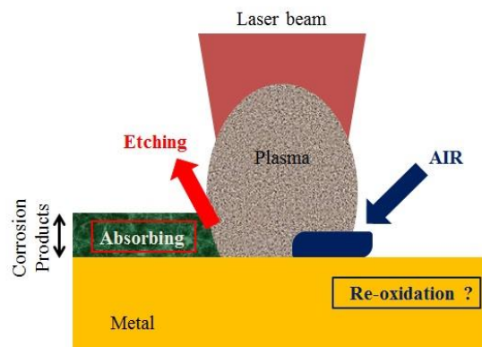
Fig. 2 Laser-material interactions.
