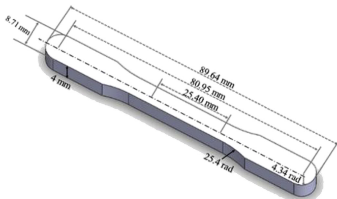
Fig. 3. Dimensional details of the flat specimen for tensile tests according to ASTM E8.
