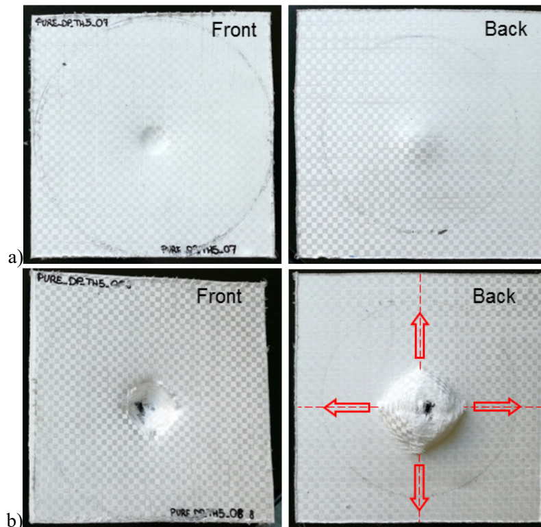
Figure 10: Photos of the samples with a thickness of 5 mm after the repetition of the impacts. Specimens tested with different impact energy are reported: a) energy level 1, b) energy level 2
