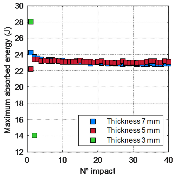
Figure 11: Experimental results for the specimens with the three considered thicknesses at the lowest energy level, as a function of the number of the impact:
