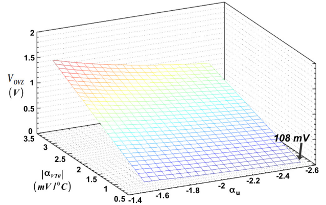
Figure 4. V_{OVZ} - ZTC overdrive voltage.
