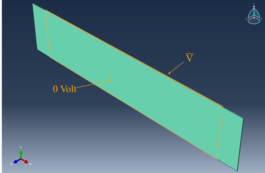
Figure 4.33: Application of the voltage to the actuators of the Abaqus models.
