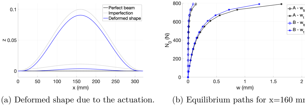
Figure 6.13: Nonlinear analysis of the beam: (a) deformed shape due to the actuation ( case B ) and for N_0 = 0 , (b) nonlinear response increasing N_0 .
