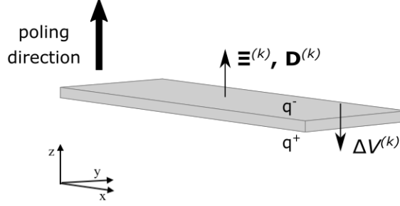
Figure 3.3: Piezoelectric layers characteristics.
