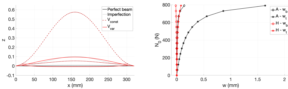
(a) Deformed shape due to the actuation. (b) Equilibrium paths for x=160 mm.
