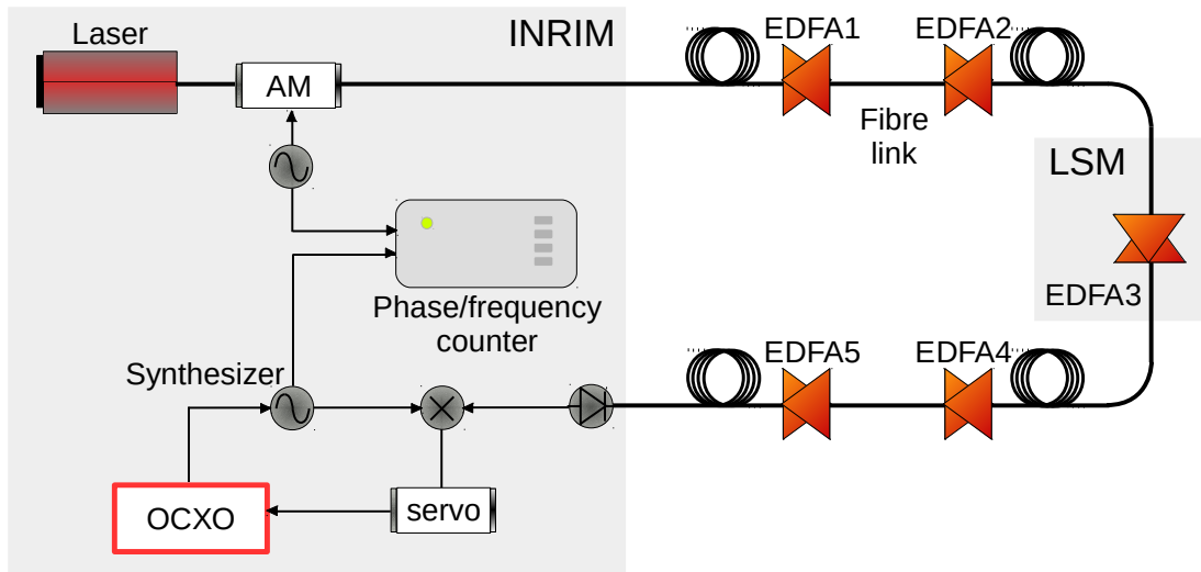
Figure 5.14: Optical and electronic apparatus for the characterization of the RF frequency dissemination over the INRIM-LSM fibre link. AM is the amplitude modulation applied to the free-running 1542 nm laser exploiting an electro-optic modulator and OCXO is the Oven-Controlled Quartz oscillator.
