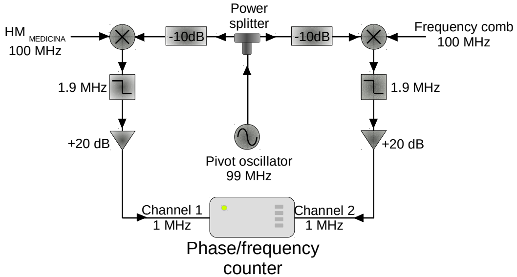
Figure 5.2: Electrical chain for the comparison of HM_{MEDICINA} and HM_{INRIM} delivered with the fibre link.
