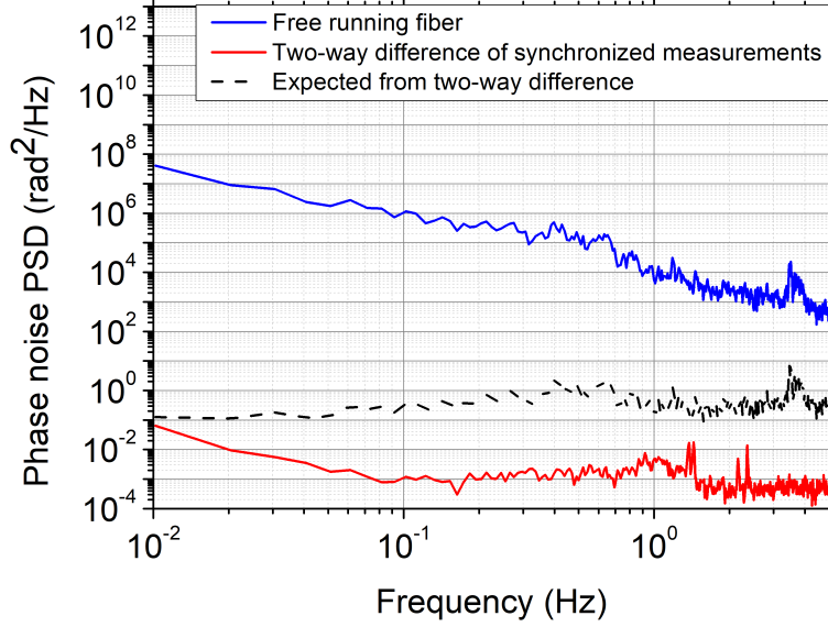
Figure 4.12: Phase noise of the 2 \times 147 km link between INRIM and Modane. Blue: noise of the free running fibre link; black: expected residual noise after two-way noise cancellation on a bidirectional fibre; red: residual noise after two-way noise cancellation on the bidirectional link based on a loop of two adjacent fibres.
