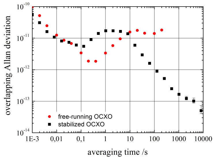
Figure 5.15: Stability in terms of Allan deviation of the OCXO noise. Red: free-running mode. Black: stability of the OCXO when locked to the optically-delivered RF signal, acquired in full bandwidth mode.
