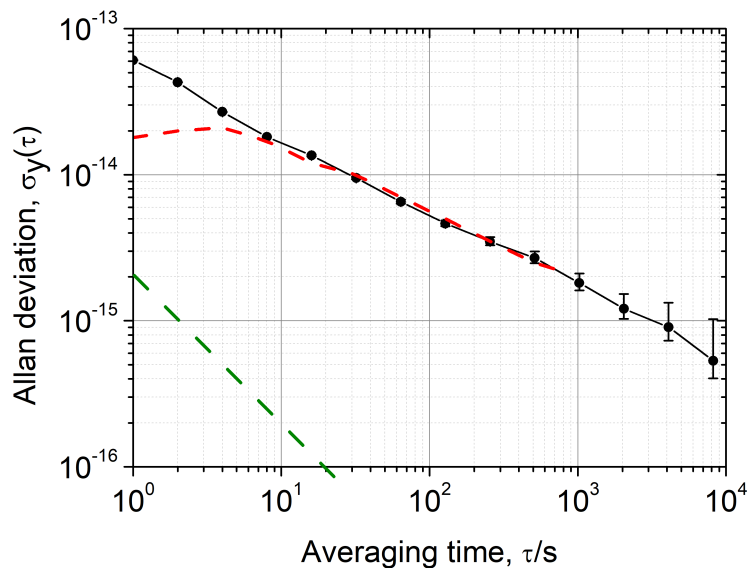
Figure 5.3: Allan deviation of the HMs comparison. Black dots: HMs comparison, HM_{MEDICINA} vs HM_{INRIM} . Red dashed line: instability of the 1542 nm laser when locked to HM_{INRIM} . Green dashed line: expected contribution from the fibre link.
