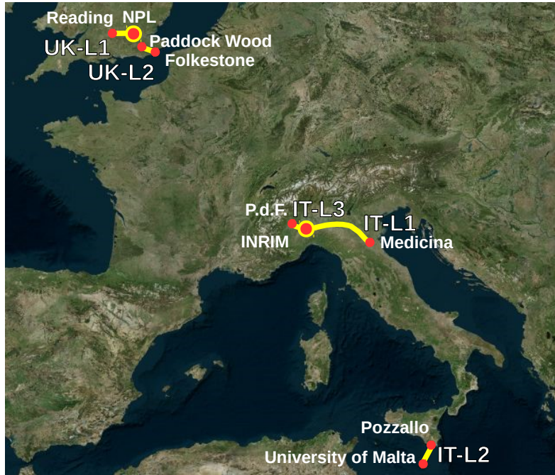
Figure 5.18: Map of the five testbeds employed for earthquakes detection. IT-L1: 535 km, connecting INRIM to Medicina. ITL2: 96.4 km, connecting Malta to Pozzallo (Sicily). IT-L3: 43 km, connecting INRIM to the amplification station of Torino via Piero della Francesca. UK-L1: 79 km, connecting NPL to the data centre in Reading. UK-L2: 75 km, connecting two amplification stations, in Paddock Wood and in Folkestone.
