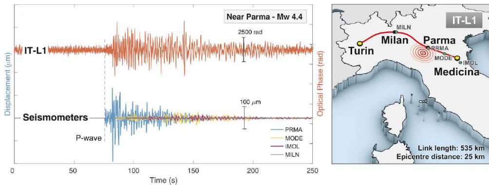
(c) Parma earthquake on 19 th November 2017. Orange: phase traces of IT-L1 link. Blue: seismograms from Parma (PRMA), Modena (MODE), Imola (IMOL) and Milano (MILN). The north-south component has been used for all seismic station data.
