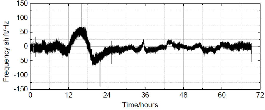
(b) Frequency shift induced by the temperature variations.
