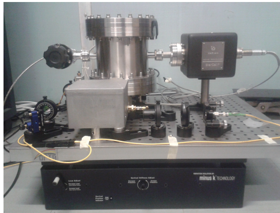
(c) Picture of the portable system: the vacuum chamber with the ion pump is placed in the centre of a 50 \times 65 cm breadboard. On the same board is mounted the optical bench for the laser alignment to the cavity.
