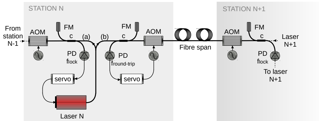
Figure 1.3: Optical and electronic apparatus of the N^{th} repetition station of cascaded links. A diode laser (Laser N) is phase-locked ( f_{lock} ) to the incoming signal from the previous station (from station N - 1 ). Part (a) is sent backwards to generate a round-trip signal in the previous station, while part (b) is sent forward to the next station. f_{round-trip} is the beat note between local and round-trip signal to compensate for the noise of the following fibre span.
