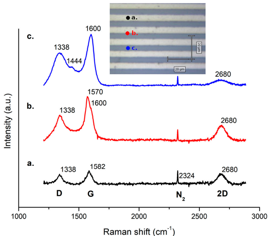
Figure 7. Raman spectra on 5 \mu\text{m} wide strips at different positions at the centre of the strip (a), on the border (b) and between two strips (c). The main peaks labels are shown. The inset shows an optical image of the sample. A graphitic carbon residual is observed in (c) while in un-patterned areas (Figure 5d) no carbon residuals are present. This shows that amorphous carbon deposition is catalysed by the presence of platinum also in a halo of 1–2 \mu\text{m} outside the pattern.
