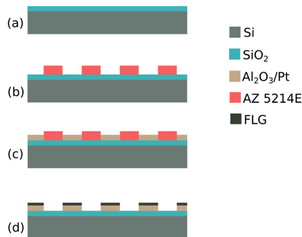
Figure 1. Process flow: (a) starting substrate, (b) photolithography, (c) \text{Al}_2\text{O}_3 /Pt deposition and lift-off, (d) graphene growth.
