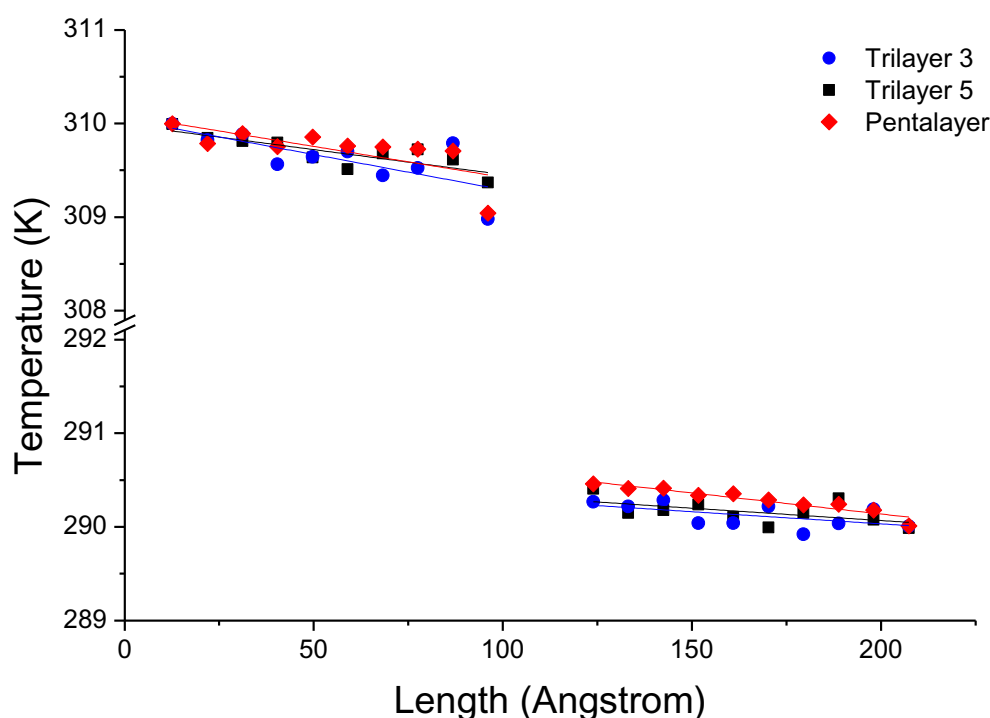
Figure 77. Thermal profile of multilayered structures bonded by C5OP linker. The temperature scale includes a 16 K break to highlight data points and linear fitting of data.
