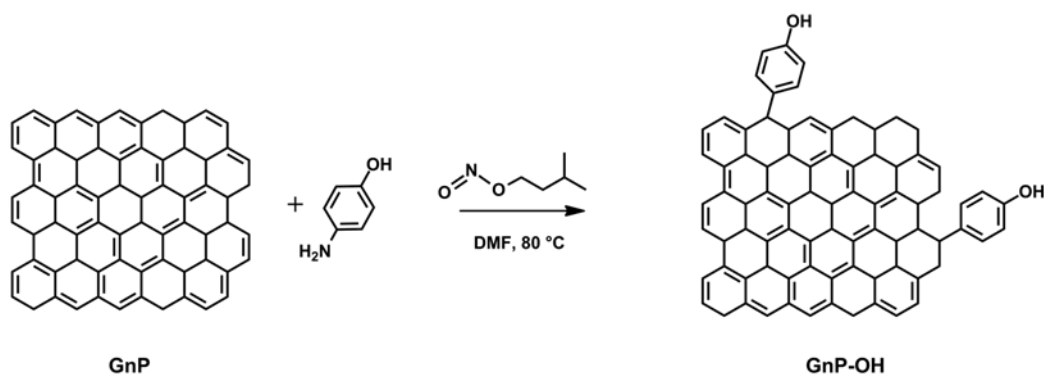
Figure 51. Edge selective functionalization with 4-aminophenol, from Bernal et al. [183].
