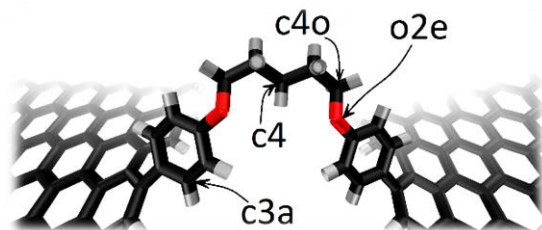
Figure 74: COMPASS© Atom types for oxygen and carbon adopted in C5OP molecular junction taken as example.
