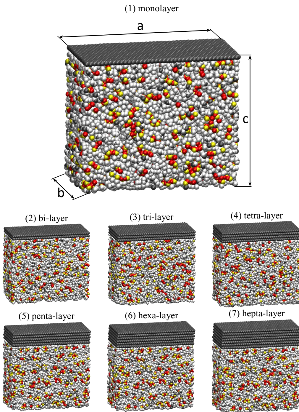
Figure 98. Model of 1 to 7 graphene layers stacked over PDMS polymer for ITC calculation. Parameters value a=99.64 , b=47.48\text{\AA} , c varied from, 84.6\text{\AA} for the monolayer (1), 88\text{\AA} for the bilayer (2), 91.4\text{\AA} for the tri-layer (3), 94.8\text{\AA} for the tetra-layer (4), 98.2\text{\AA} for the penta-layer (5), 101.6\text{\AA} for the hexa-layer and 105\text{\AA} for the hepta-layer. Wrapped view with VMD, color codes: carbon in grey, hydrogen in white, oxygen in red and silicon in yellow.
