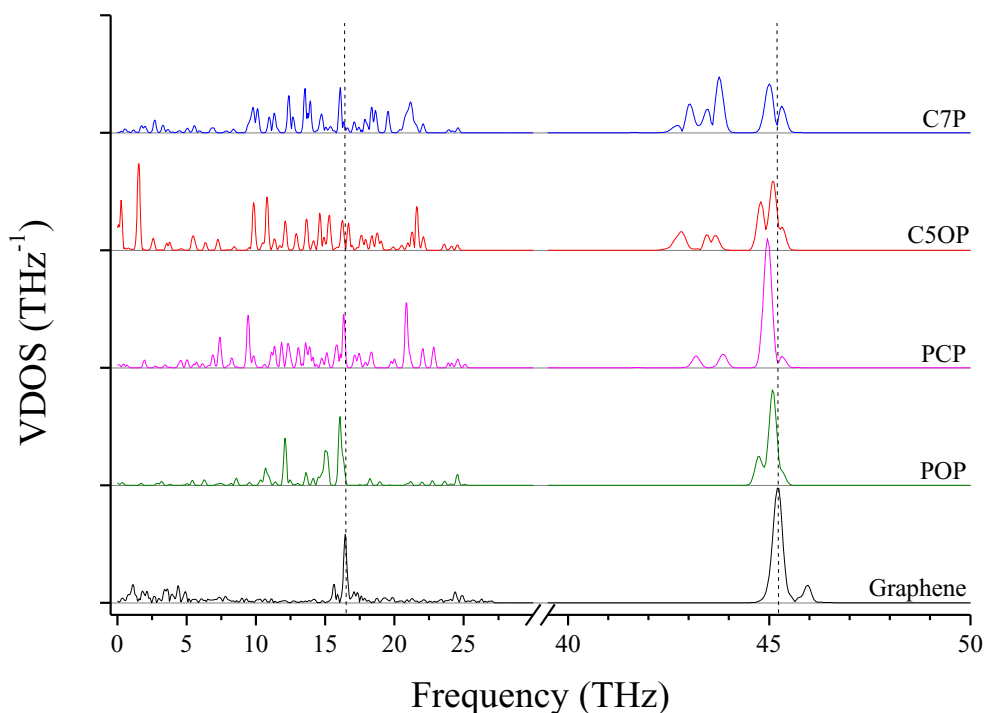
Figure 73. VDOS for molecular junctions with/without ether bridge, the scale in 40-50 THz is magnified by a factor of three for clarity. Dashed lines highlights the most intense graphene peaks at 16.5 THz and 45.2 THz (G-peak).
