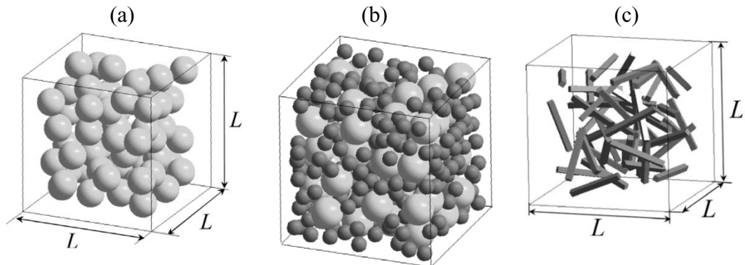
Figure 37. Three different RVE's developed from Sanada and coworkers with different particles. (a) with one type of sphere and (b) two types of spheres acting as fillers.(c) Modelled nanotubes in RVE. Reprinted from [160], with permission from Elsevier.
