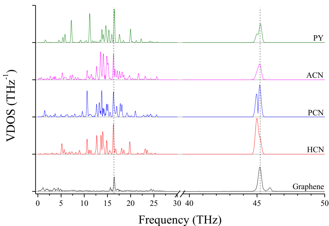
Figure 85. VDOS in acenes, scale in 40-50 THz is magnified by a factor of three. Dashed lines highlights the most intense graphene peaks at 16.5 THz and 45.2 THz (G-peak). PY is added for the sake of comparison.
