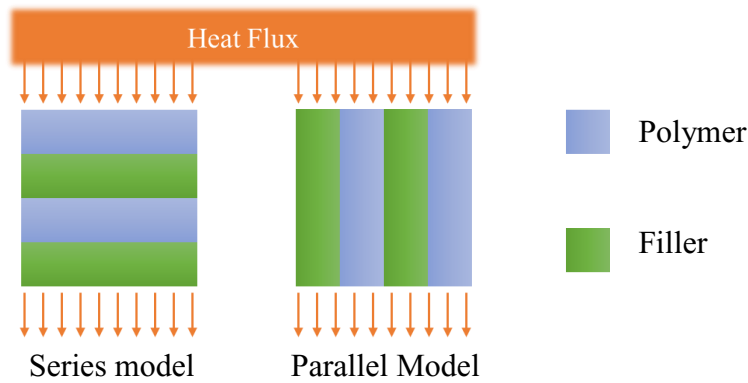
Figure 11. Series and parallel models for predicting thermal conductivity in composites.
