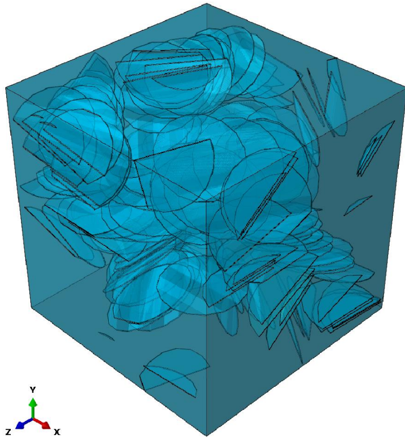
Figure 46. Example of composite RVE for FEM analysis: in this RVE the filler is represented by 150 flat disks of aspect ratio 1:100 in a 4% of volume concentration.
