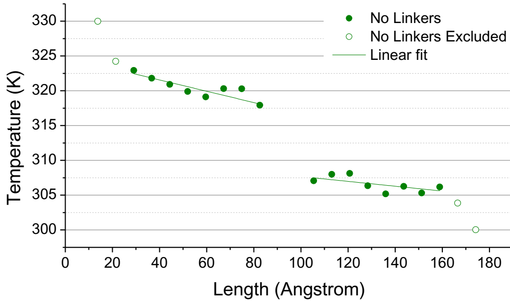
Figure 92. Thermal slabs temperature as a function of the spatial arrangement for polymer embedded graphene platelets without linkers.
