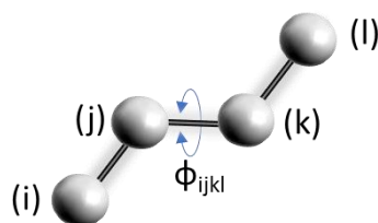
Figure 7. Dihedral angle in Molecular Dynamics Force Field.
