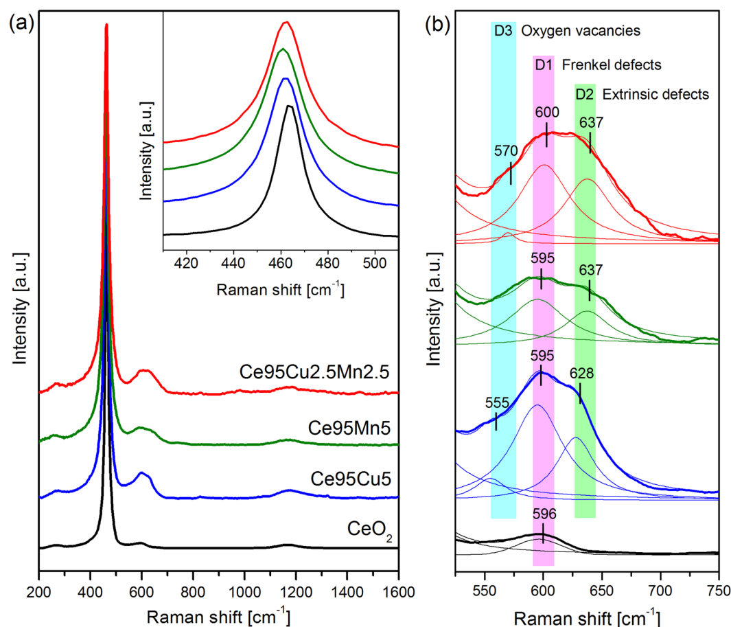
Figure 2. Average Raman spectra of the four catalysts at RT (a), with magnifications of the F_{2g} peak (inset) and of the defects band region (b). The traces obtained by curve fit and deconvolution of the defect-induced band are also reported (thin lines). All the spectra were normalized to the F_{2g} band.
