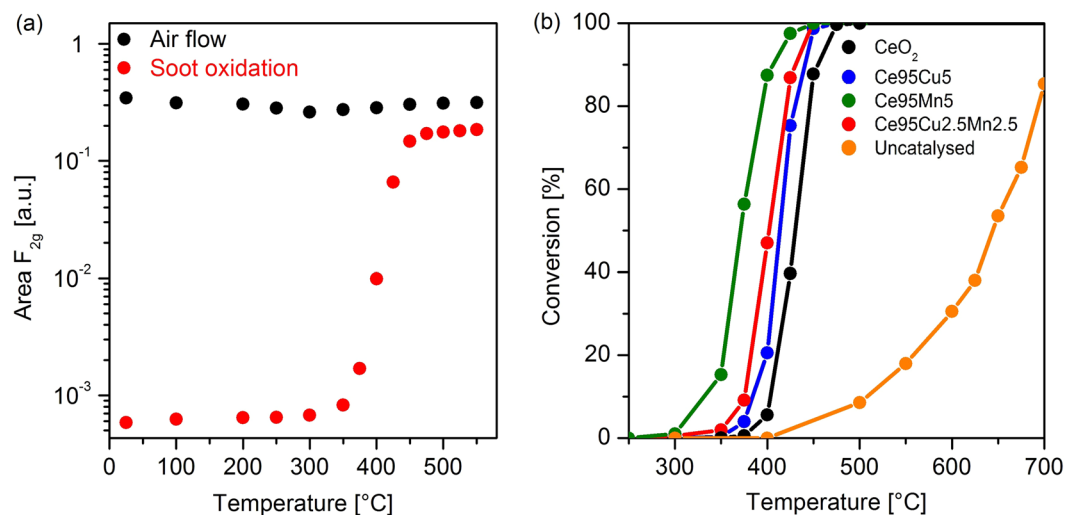
Figure 7. Variation of the F_{2g} peak area as a function of temperature during the analysis in air flow (black dots) and during soot oxidation (red dots) on the \text{CeO}_2 catalyst (a); the area of the F_{2g} band has been normalized to the acquisition parameters and to the area of the main band of the internal Si reference. Soot conversion curves obtained from the Raman spectra collected during the in situ tests over the four catalysts and for the uncatalysed reaction (b); the last curve was obtained as detailed in the caption of Supplementary Fig. S6.
