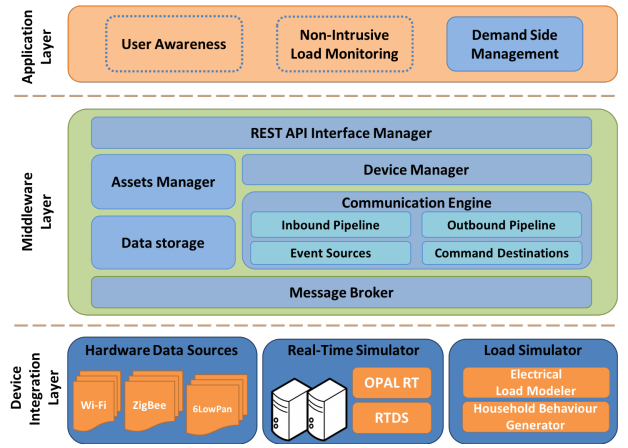
Fig. 1. Scheme of Flexmeter platform.
