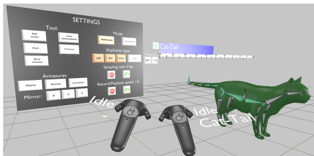
FIGURE 2. First-person view of the VR Blender immersive interface during user interaction; on the left side, widgets introduced to manage armature deformation-based animation tasks are shown. More information on other elements can be found in [9].
