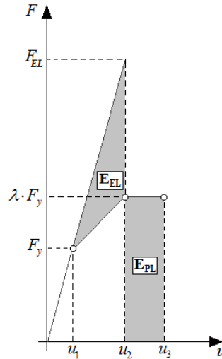
Figure 5. Equivalent elastic energy ( E_{EL} ) and elasto-plastic energy ( E_{PL} ) of the system.
