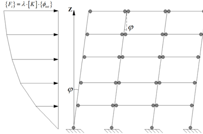
Figure 4. Global collapse mechanism.
