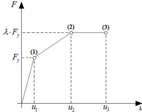
Figure 2. Trilinear backbone curve.
