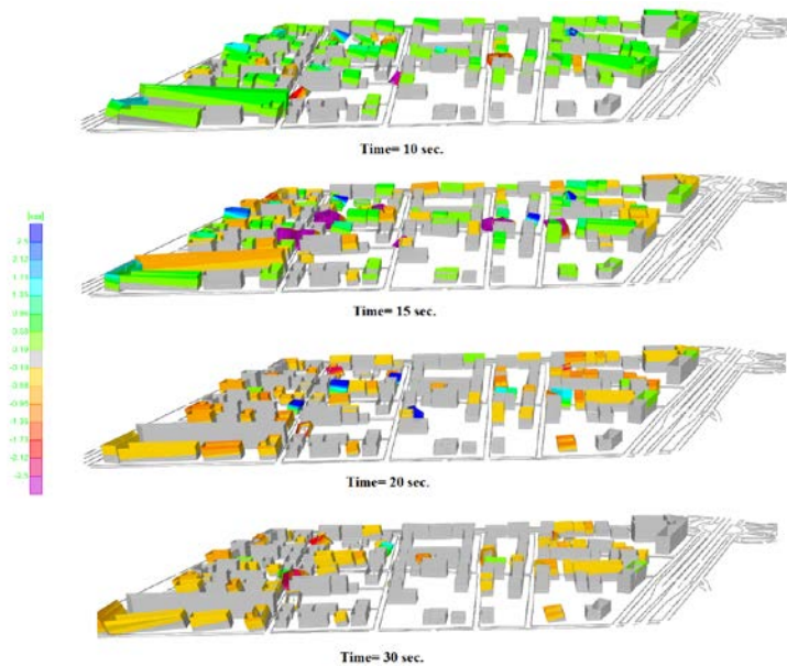
Figure 6. Displacement contours at four different time steps.
