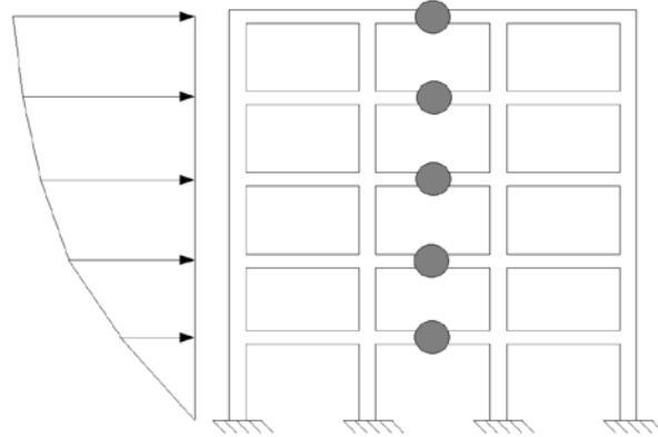
Figure 3. Concept of nonlinear MDOF system.
