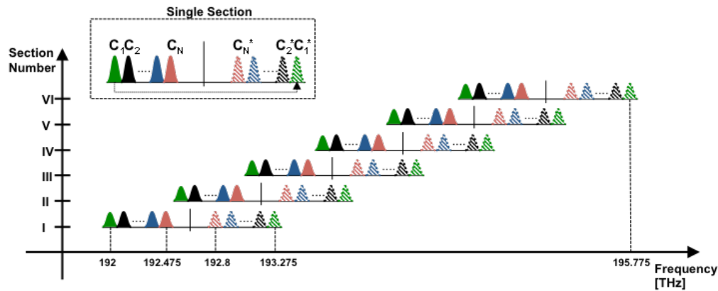
Fig. 6. Frequency sections of transmitted and conjugated channels.
