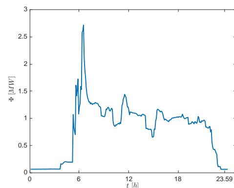
Figure 9. Heat flux required by the distribution network.
