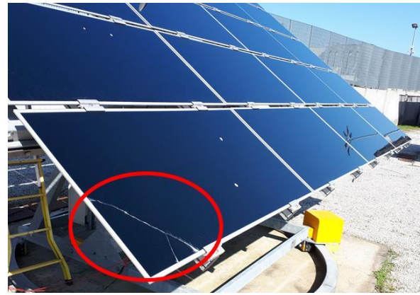
Figure 7. Detail of the broken module in plant E_{ts} (CdTe thin-film on an x-y tracking system).
