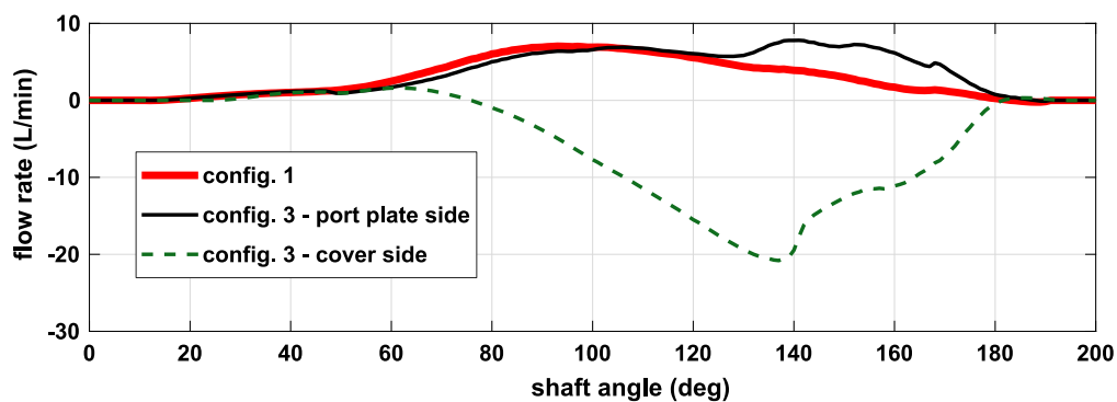
Figure 8. Radial flow rate through the millings on the stator.
