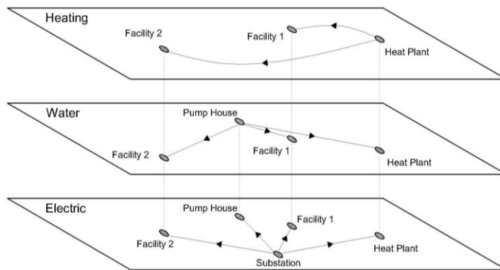
Figure 3: Example of layer subdivision for interdependent networks
