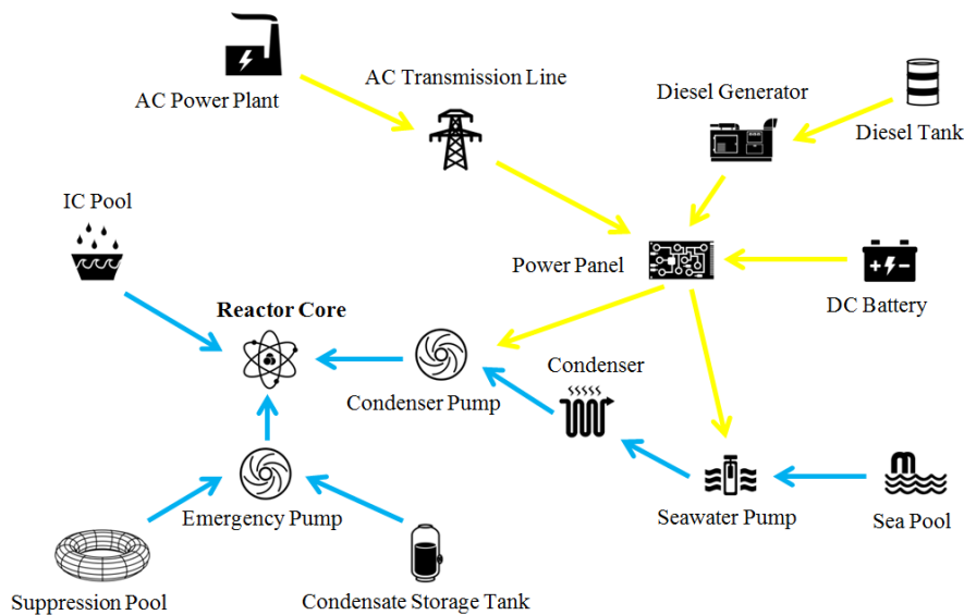
Figure 5: Simplified model for lifelines serving a nuclear power plant
