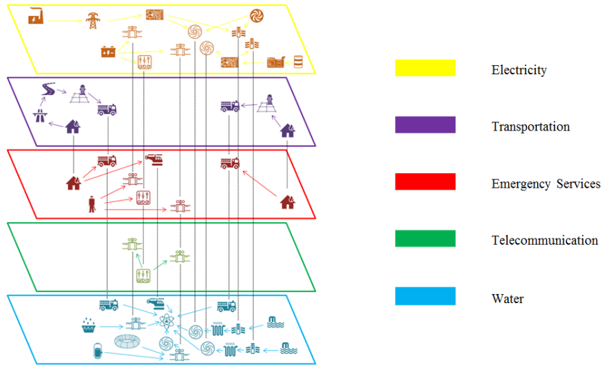
Figure 6: Interdependent layers of the detailed model for lifelines serving a nuclear power plant
