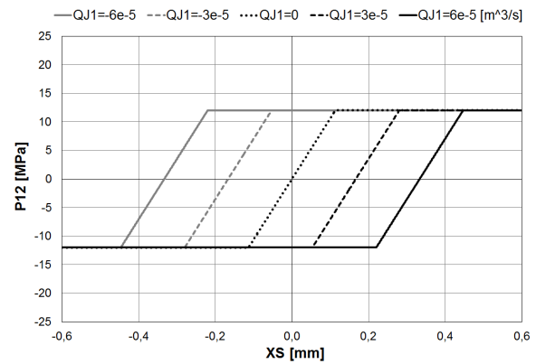
Fig. 27 MODEL C2 – CLk = 2 \cdot 10^{-13} m³/s/Pa and PSR = 12 MPa
