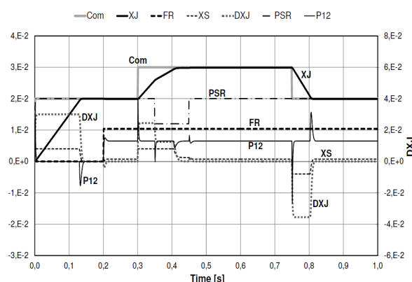
Fig. 35 EHA dynamic response – MODEL A
