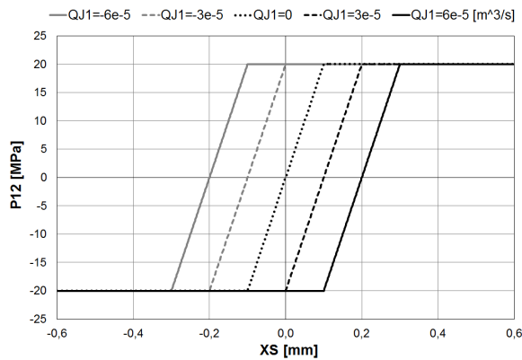
Fig. 28 MODEL C3 – CLk = 0 m 3 /s/Pa and PSR = 20 MPa
