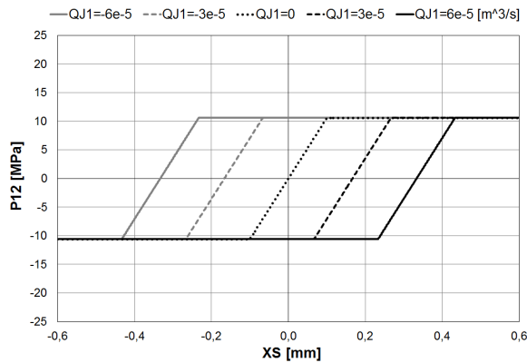
Fig. 24 MODEL C1 – CLk = 2 \cdot 10^{-13} m³/s/Pa and PSR = 12 MPa
