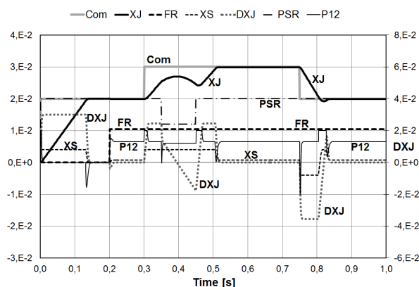
Fig. 38 EHA dynamic response – MODEL C2
