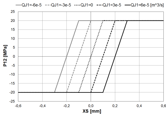
Fig. 25 MODEL C2 – CLk = 0 m³/s/Pa and PSR = 20 MPa
