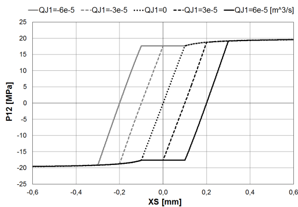
Fig. 29 MODEL C3 – CLk = 2 \cdot 10^{-13} m 3 /s/Pa and PSR = 20 MPa
