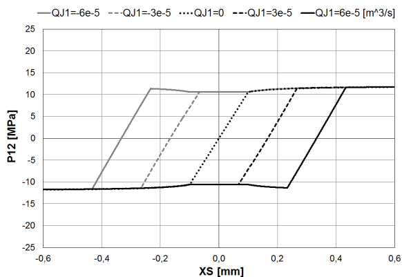
Fig. 30 MODEL C3 – CLk = 2 \cdot 10^{-13} m 3 /s/Pa and PSR = 12 MPa
