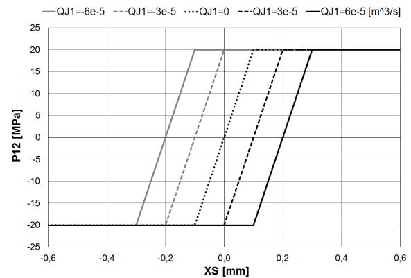
Fig. 31 MODEL C4 – CLk = 0 m 3 /s/Pa and PSR = 20 MPa
