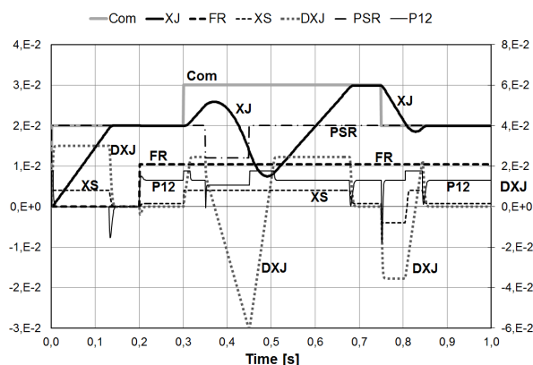
Fig. 37 EHA dynamic response – MODEL C1
