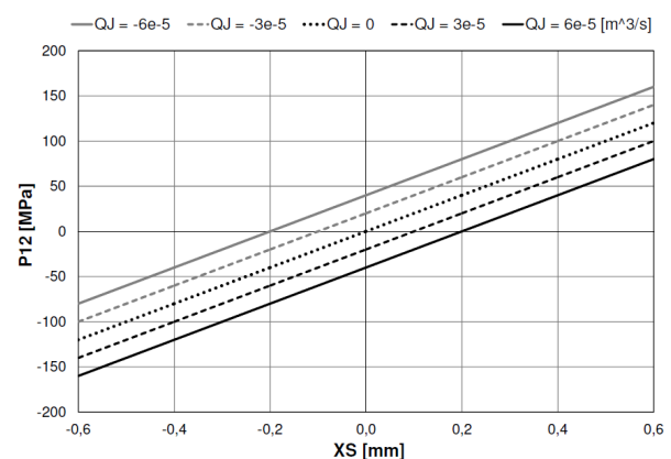
Fig. 18 MODEL A in case of CLk = 0 \text{ m}^3/\text{s/Pa} and PSR = 20 \text{ MPa}
