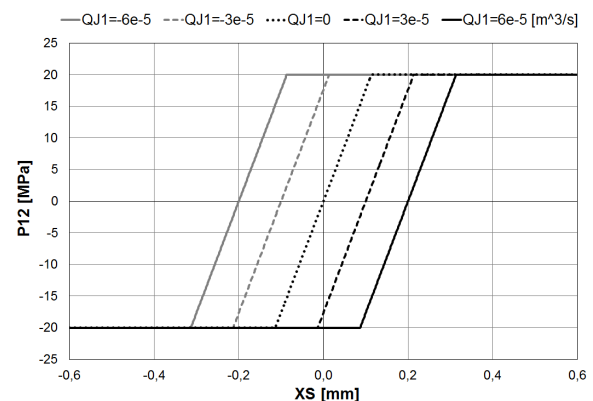
Fig. 32 MODEL C4 – CLk = 2 \cdot 10^{-13} m 3 /s/Pa and PSR = 20 MPa
