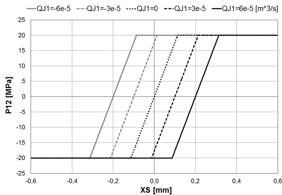
Fig. 26 MODEL C2 – CLk = 2 \cdot 10^{-13} m³/s/Pa and PSR = 20 MPa
