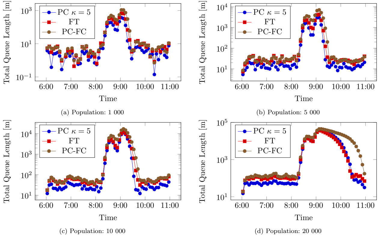
Fig. 6. Comparison of the proportional control with dynamic cycle length (PC) with \kappa = 5 , proportional control with fixed cycle length (PC-FC) and fixed signal timing (FT) for the four different scenarios. To improve readability the queue lengths are averaged over a five-minute interval and the y-axis is in log-scale.
