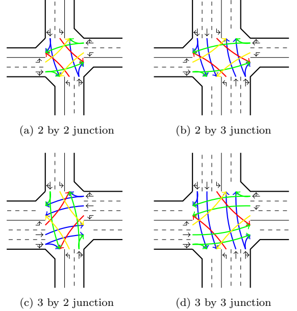
Fig. 2. The four different types of junctions.
