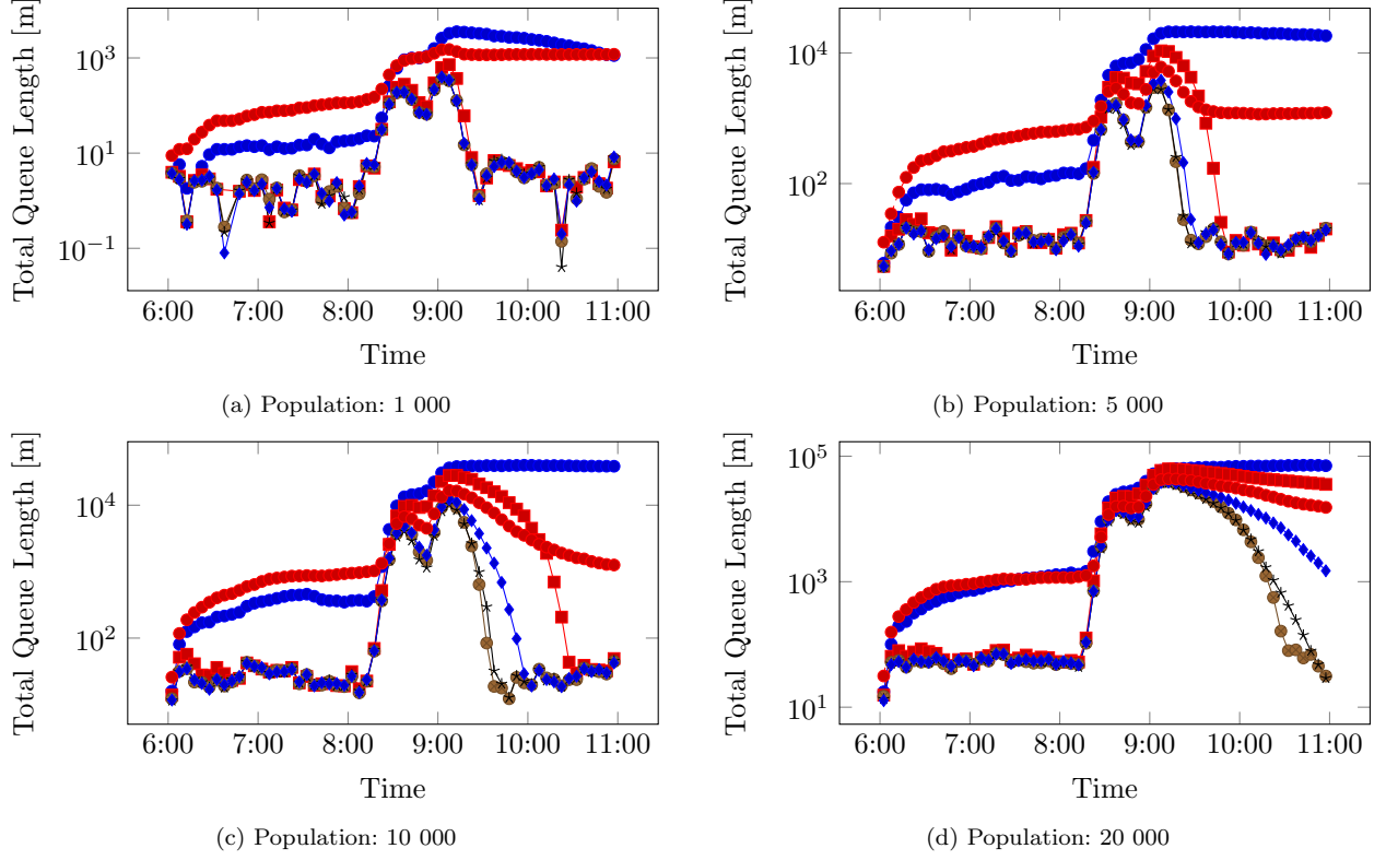
Fig. 5. The total queue lengths for different choices of \kappa for the four different scenarios. To improve readability, the queue lengths are averaged over a five-minute interval and the y-axis is in log-scale. The values of \kappa are 0.1 (—●—), 1 (—■—), 5 (—●—), 10 (—*—), 20 (—◆—) and 40 (—◆—).
