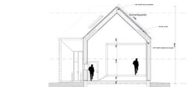
► Fig. 3: Vertical section of the ZEB Test Cells Laboratory with one test cell and one guarded volume.
