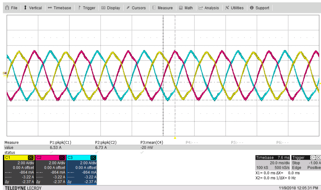
Figure 9. Motor currents at 500 rpm.
