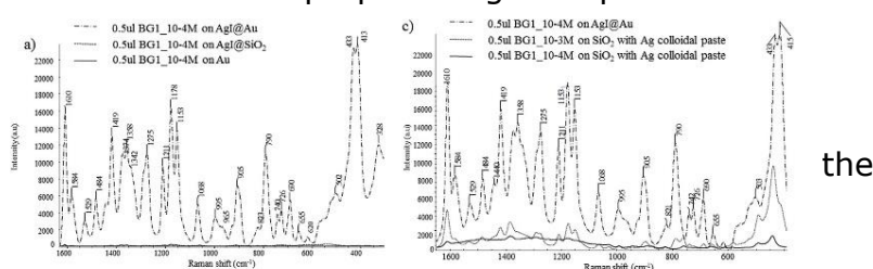
Figure 1. Spectra of BG1 extracted dye from wool with SERS and MU-ATR after TLC development.
