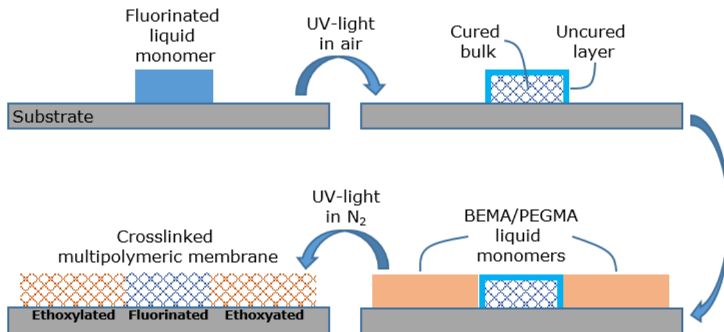
Figure 51: Scheme of the preparation process of the multifunctional polymer electrolyte. Reprinted with permission. Copyright 2018, Elsevier.
