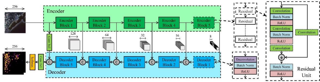
Figure 37 Proposed Network include encoder (top) and decoder (bottom) modules, an encoder and a decoder block are detailed in dashed boxes
