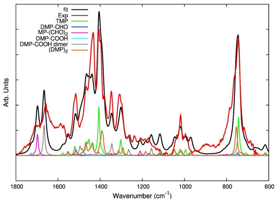
Figure 7. Result of the fitting of the experimental spectrum (red line) of a TMP sample after thermal treatment (reference spectrum of modified TMP (sample treated at 130\text{ }^{\circ}\text{C} , spectrum recorded after TMP evaporation). The fitting curve (black line) is obtained as a weighted sum of theoretically predicted spectra for some model molecules (oxidized species and dimer) illustrated in Table 1. The spectra included in the fitting are displayed in different colors: each spectrum is multiplied by a factor proportional to the weight adopted in the fit.
