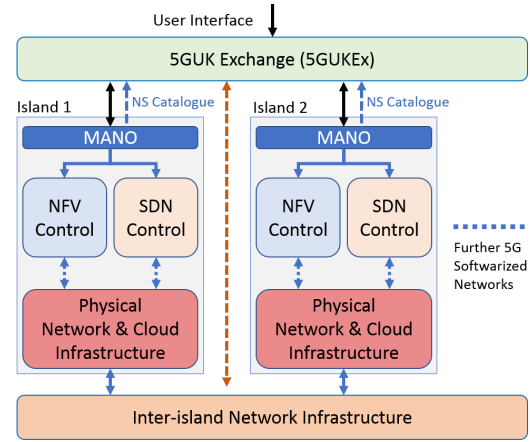
Fig. 1: 5GUK Exchange Architecture
