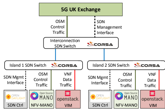
Fig. 3: 5GUKEx: Demo Setup
