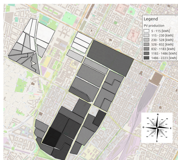
(b) Total PV generation (sunny day)
