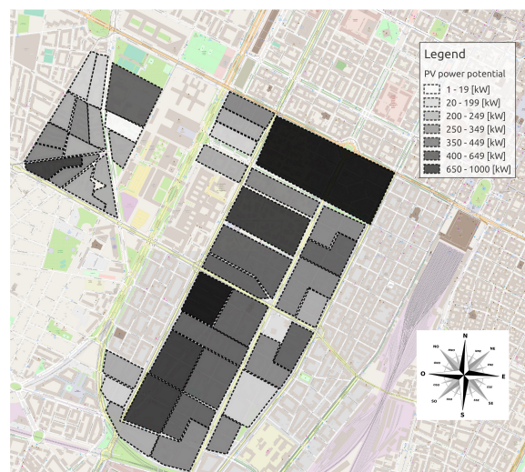
(a) PV power potential (sunny day)
