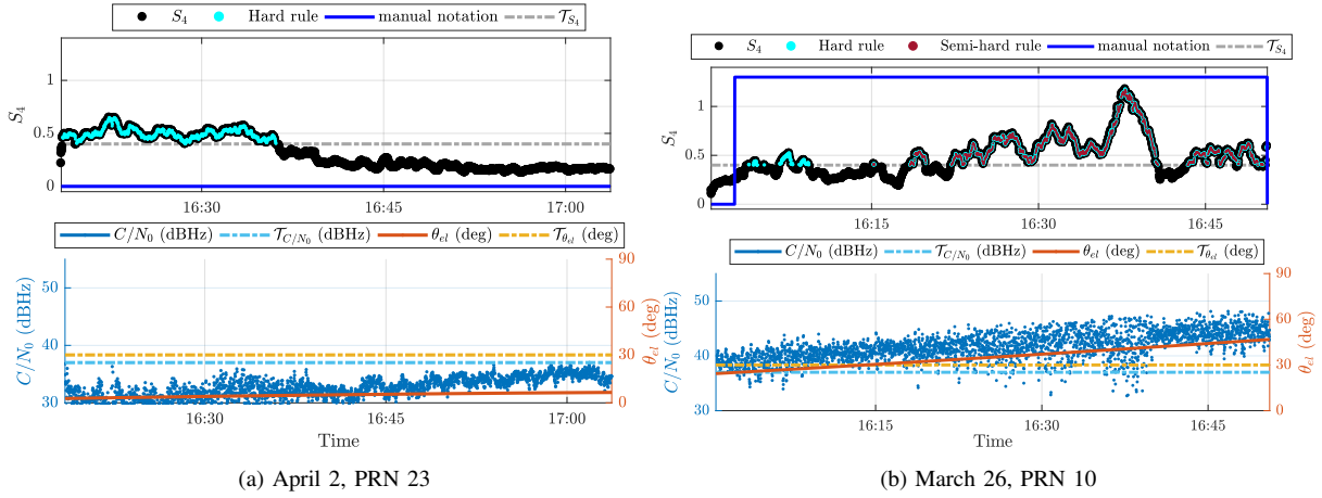
Fig. 3. Comparison of traditional scintillation detection methods for two different scintillation events. Top panels report the trend of the S_4 , the manual annotation, the detection results of the Hard and Semi-hard rules and the value of the S_4 threshold \mathcal{T}_{S_4} = 0.4 . Bottom panels report the elevation and C/N_0 trends, and their respective thresholds used in traditional rules, \mathcal{T}_{\theta_{el}} = 30^\circ and \mathcal{T}_{C/N_0} = 37 dBHz.
