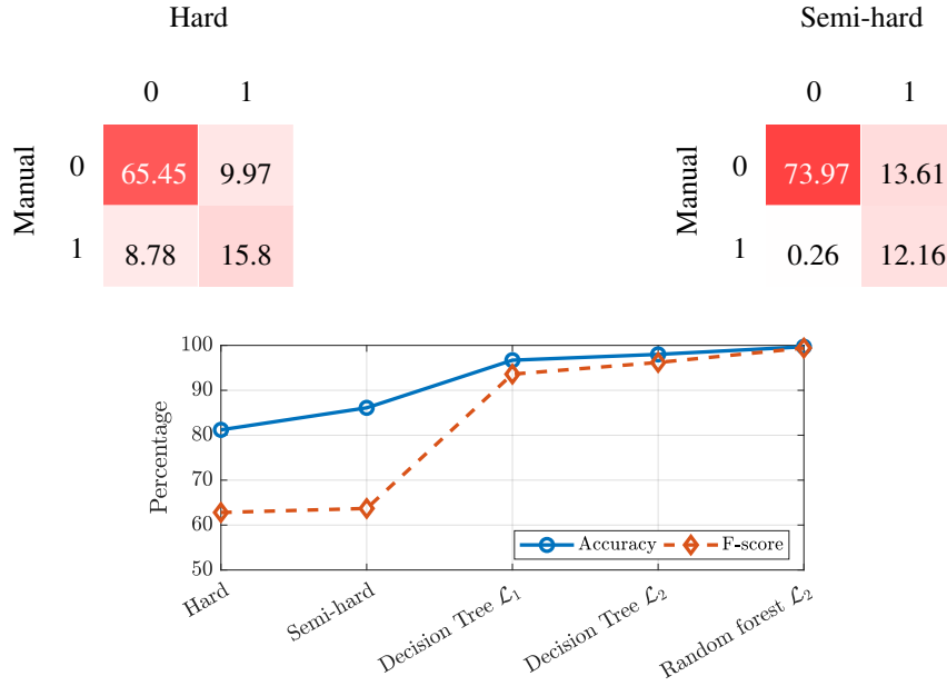
Fig. 8. Summary of the accuracy and F-score obtained for the different scintillation detection techniques presented.
