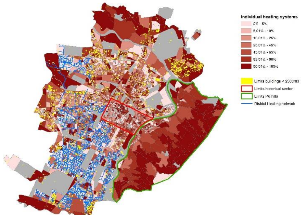
Figure 6: Data about individual heating systems and the territorials and economical constrains for the DH network expansion
