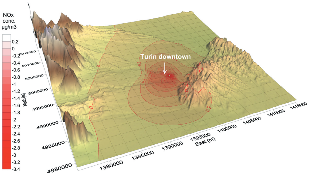
Figure 4: \text{NO}_x average concentration difference at ground level between future and present scenarios in the entire modelling domain. The average is calculated over the six coldest months of the year (October to March).
