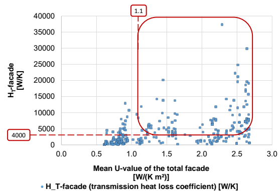
Fig. 2 – Qualitative overview of buildings with a high total facade U-Value and a big transmission heat loss coefficient H_T
