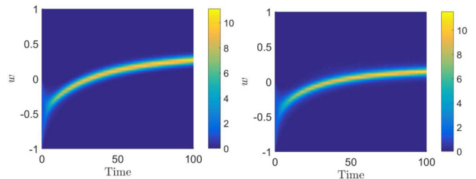
FIG. 8. Test 2, Sec. IV B. Time evolution of the marginal opinion density f(t, w) in the time interval [0,100] for power-law (left) and exponential (right) connectivity distribution.
