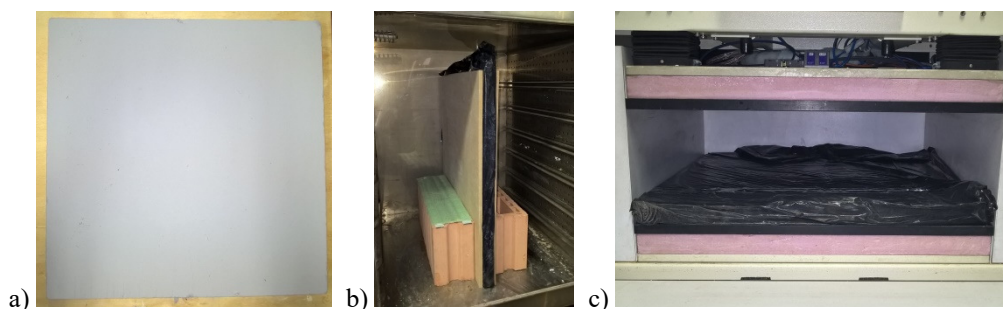
Figure 82: APM rigid board. a) sample; b) drying phase; c) plastic wrapping
