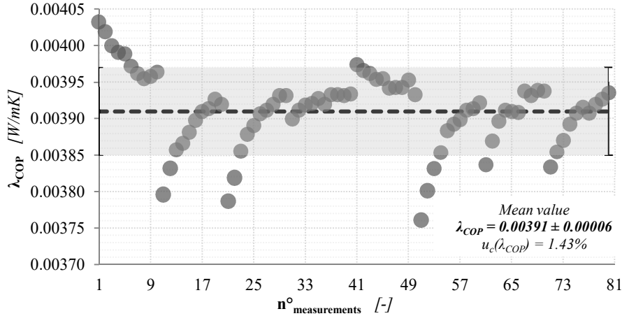
Figure B. 25: \lambda_{COP} -values assessed by means of HFM-1 apparatus (Sample: FS based VIP 20 mm thick, \vartheta_{avg} = 23^\circ\text{C} , \Delta\vartheta = 10^\circ\text{C} )
