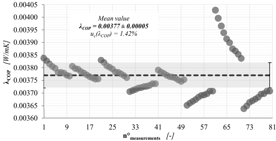
Figure B. 23: \lambda_{COP} -values assessed by means of HFM-1 apparatus (Sample: FS based VIP 20 mm thick, \vartheta_{avg} = 10^\circ\text{C} , \Delta\vartheta = 30^\circ\text{C} )
