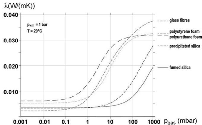
Figure 14: Thermal conductivity of different insulation materials as a function of the internal residual pressure [28]
