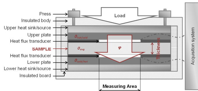
Figure 30: Single specimen symmetrical HFM apparatus
