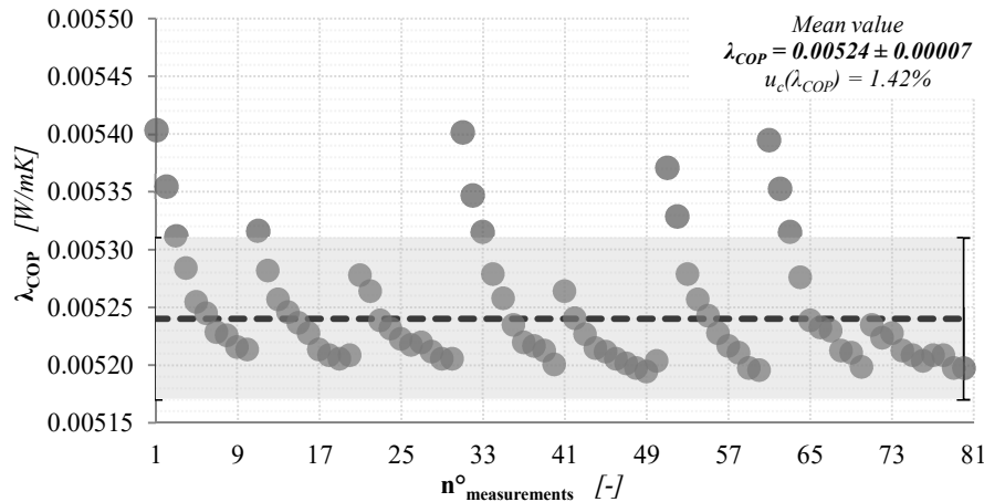
Figure B. 44: \lambda_{COP} -values assessed by means of HFM-1 apparatus (Sample: FS based VIP 30 mm thick, \vartheta_{avg} = 23^\circ\text{C} , \Delta\vartheta = 40^\circ\text{C} )
