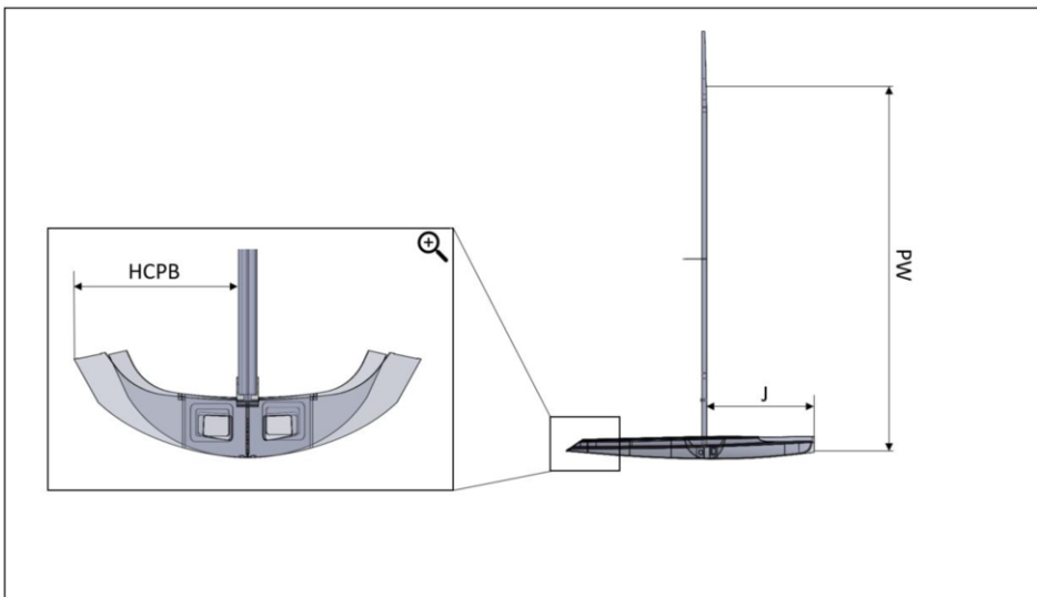
Figure 4. Characteristic dimensions
