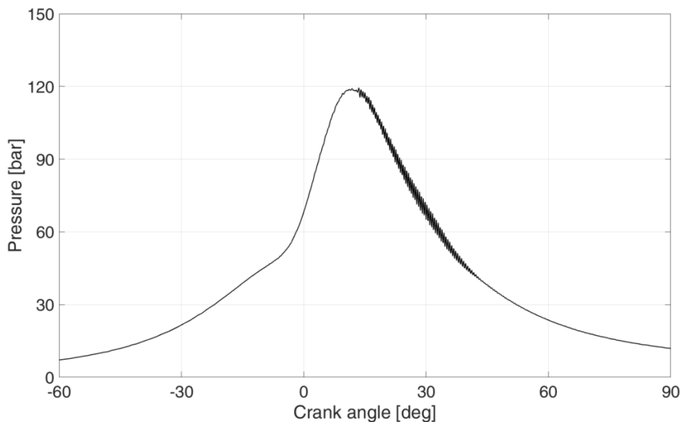
Figure 5.5: Ringing cycle
