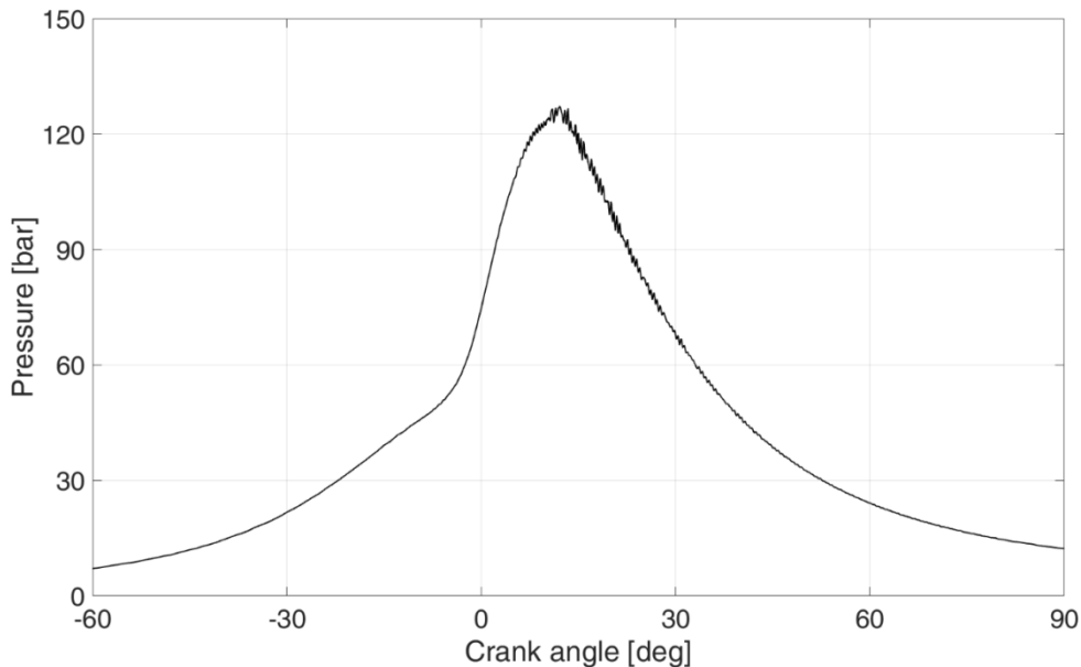
Figure 5.4: Knocking cycle
