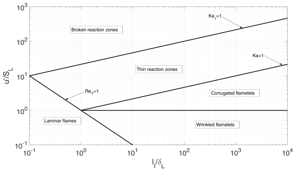
Figure 5.3: Borghi diagram [5]
