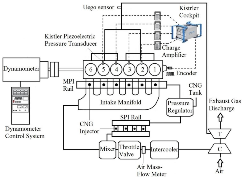
Figure 4.1: Engine set-up [14]
