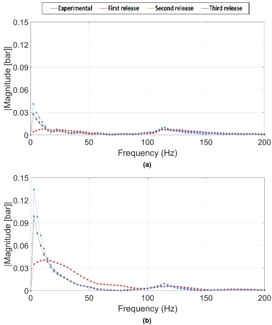
Figure 3.8: Comparison of single-sided spectrum between experimental data and simulation results for two single injection tests: (a) ET=4000 \mu s , (b) ET=14000 \mu s . [14]
