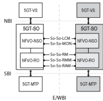
Figure 2: 5GT-SO functional architecture
