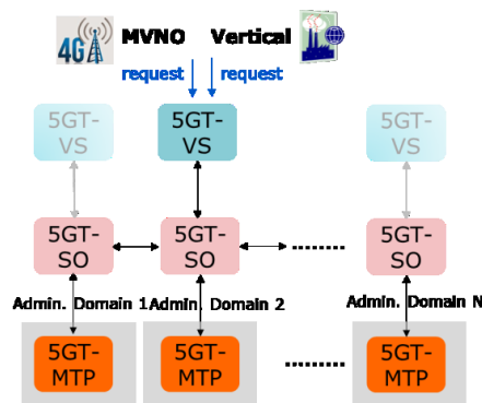
Figure 1: The 5G-TRANSFORMER concept
