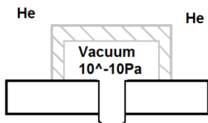
Figure 14. Gas tightness test for half box.
