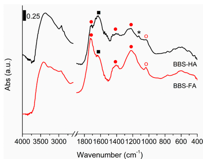
Figure 1. Absorbance FTIR spectra in the 4000\text{--}400\text{ cm}^{-1} range of BBS-HA (solid black curve), and BBS-FA (solid red curve). The main relevant peaks are labeled. Legend: aromatic C=C (black square), O-containing functional groups (red circle), polysaccharide-like impurities (white circle), and alcoholic/ether C–O (black star).
