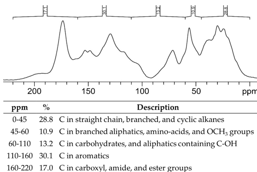
Figure 2. ^{13}\text{C} CPMAS solid-state NMR spectrum of BBS-HA ( top ), assignments and relative area calculated from the NMR spectrum ( bottom ).
