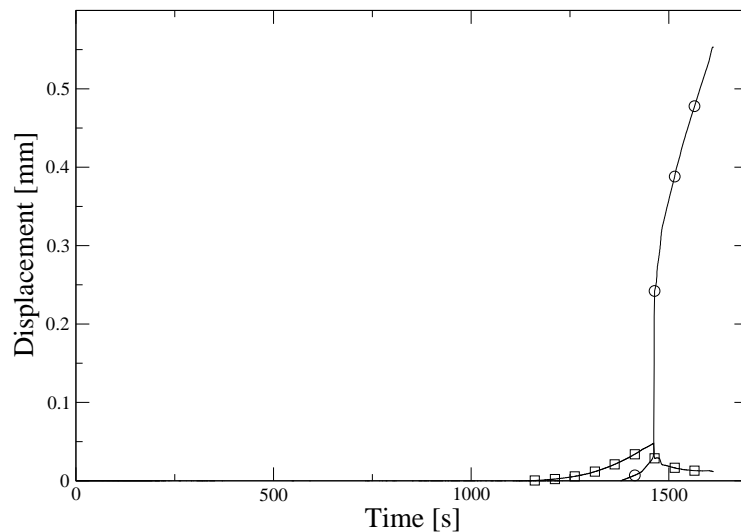
Figure 10. Experimental results for the second specimen: (○) transducer SP1, (□) transducer SP5
